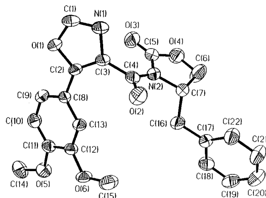
Figure 1. Computer drawing of (S)-2 (C 22 H 20 N 2 O 6 ; fw, 408.4; monoclinic, P 2 1 2 1 2 1 ; colorless; a = 7.863(1) Å, b = 10.059(1) Å, c = 25.218(3) Å; Z = 4; R = 3.85%; GOF = 1.82). Ellipsoids are drawn at the 50% probability level.
